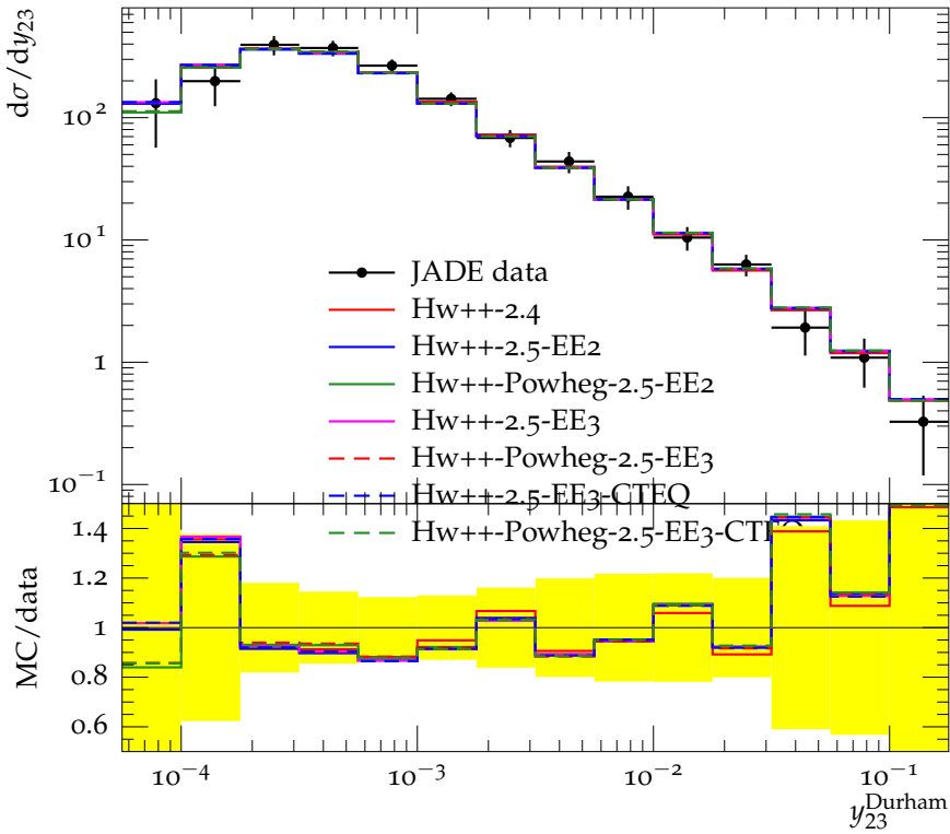
Differential 2-jet rate with Durham algorithm (183 GeV)
