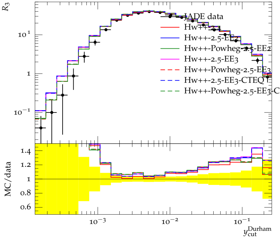
Integrated 3-jet rate with Durham algorithm (44 GeV)
