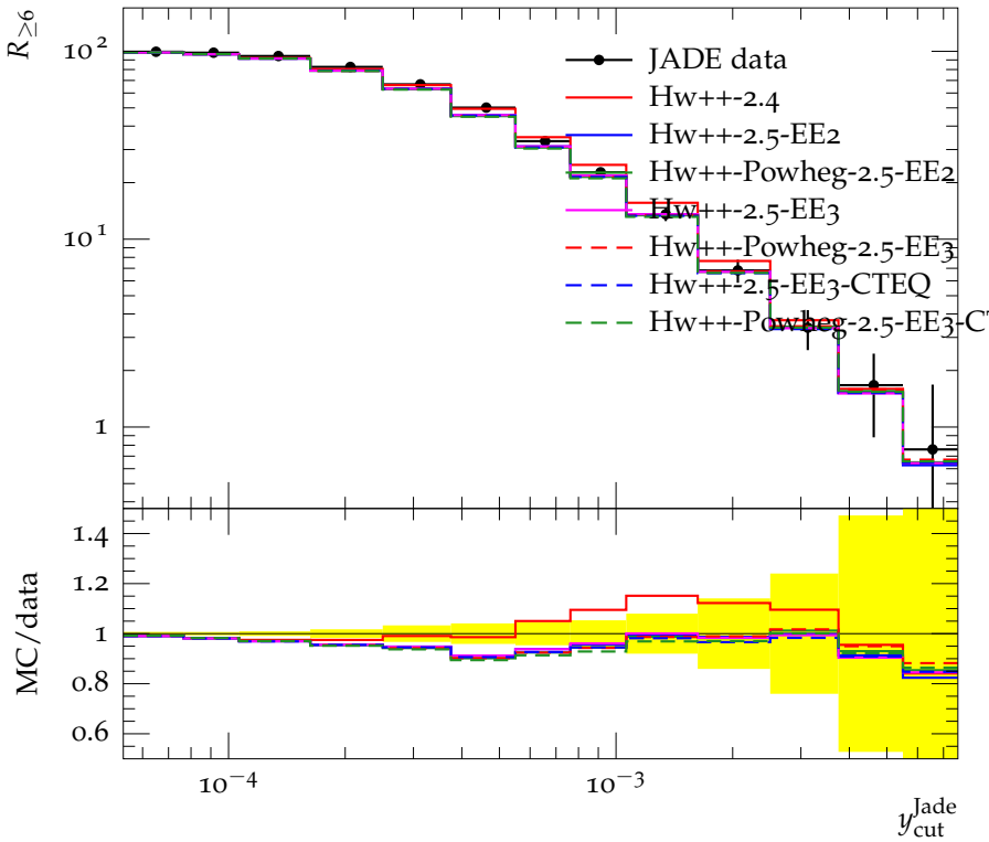
Integrated \geq 6 -jet rate with Jade algorithm (189 GeV)
