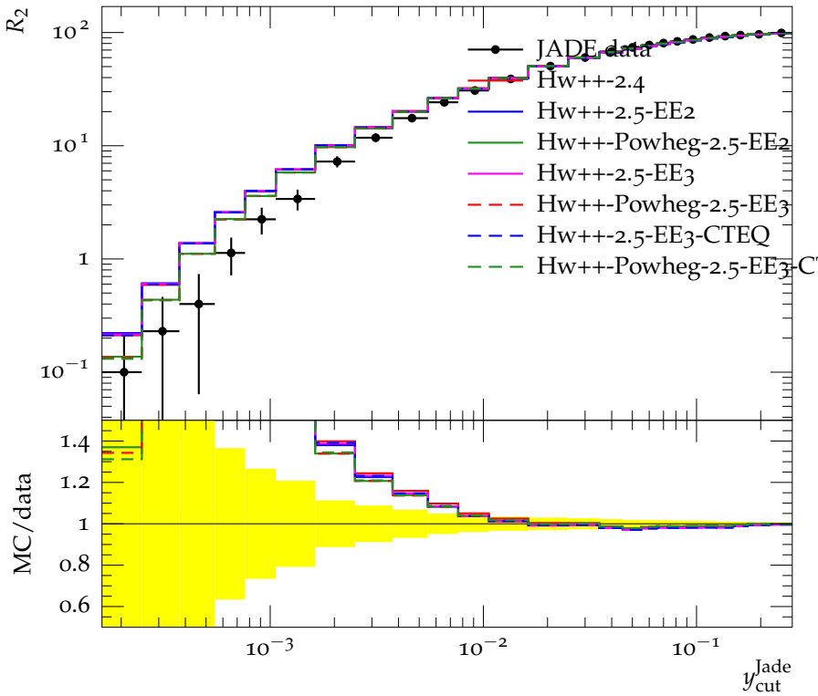
Integrated 2-jet rate with Jade algorithm (189 GeV)
