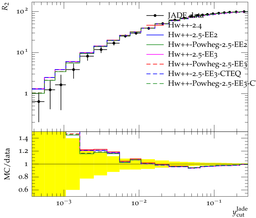
Integrated 2-jet rate with Jade algorithm (183 GeV)
