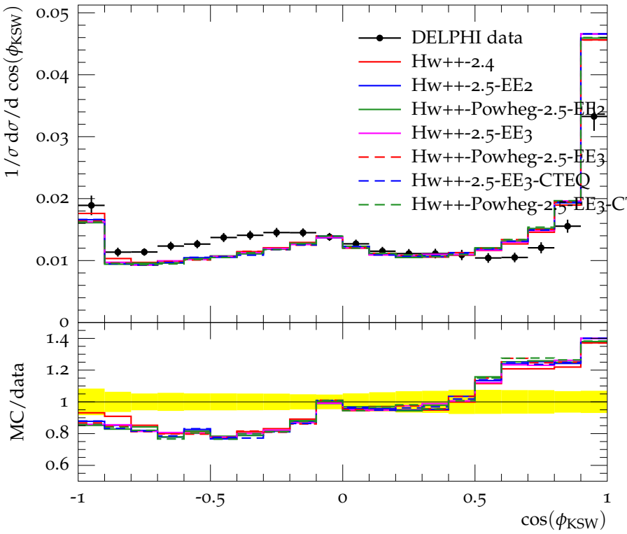
Körner-Schierholz-Willrodt \cos(\phi_{\text{KSW}}) , Jade y_{\text{cut}} = 0.015
