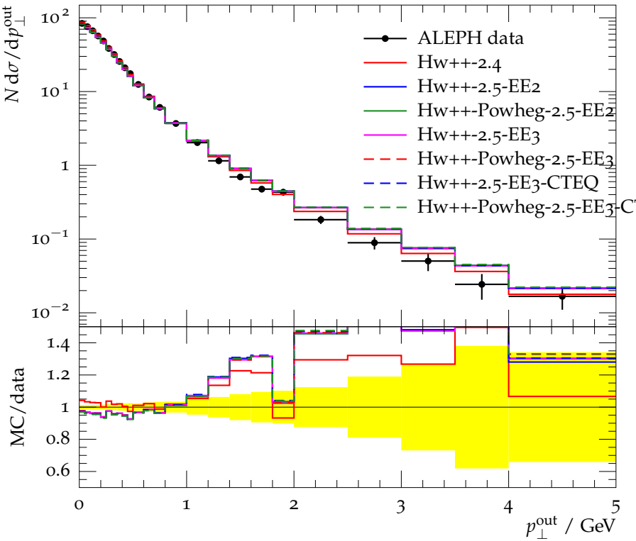
Out-of-plane p_{\perp} in GeV w.r.t. thrust axes ( E_{\text{CMS}} = 206 GeV)
